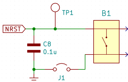
Figure 4.7. Microcontroller Reset Button
